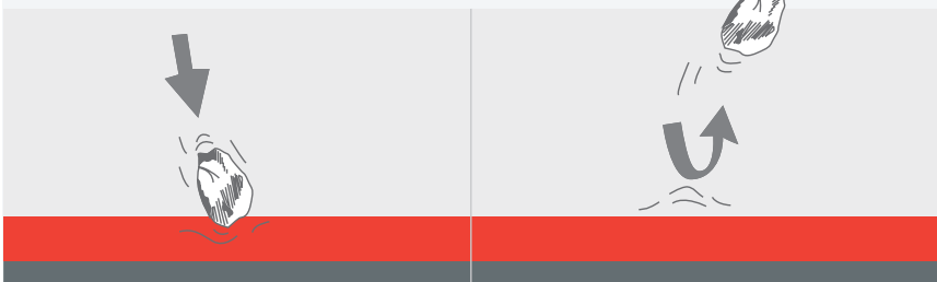
Abrasive particle striking resilient rubber surface. Rubber deforms under load and returns most of kinetic energy to the particle without rate of wear experienced above.
